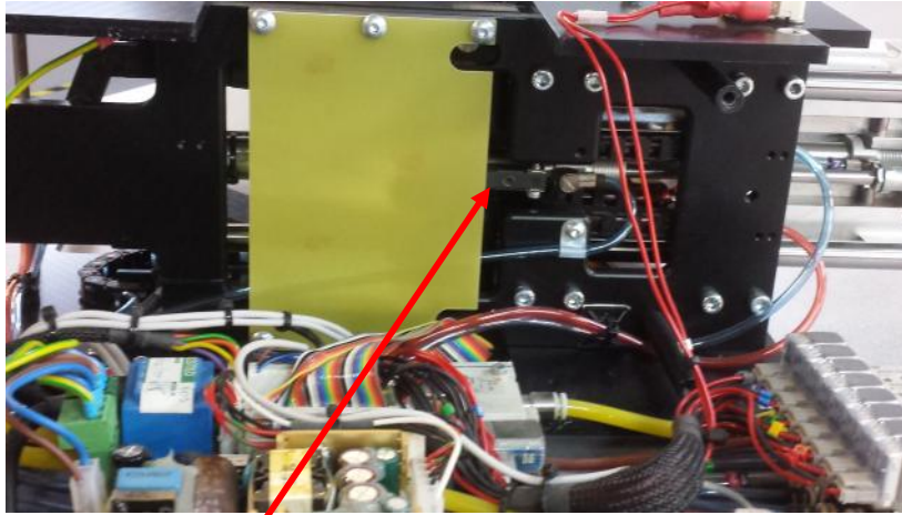
Cylinder sensor location ( front sensor)
